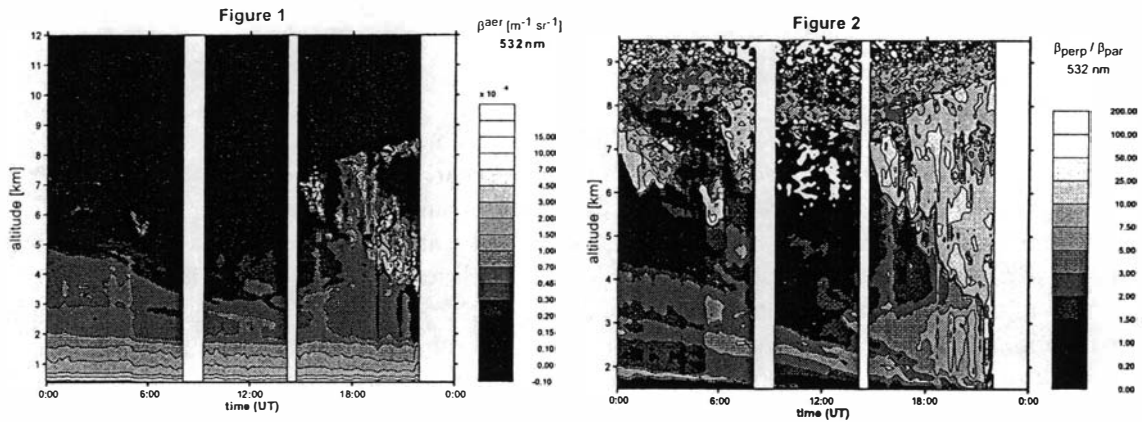
March 5 th : backscatter coefficient in laser polarisation
