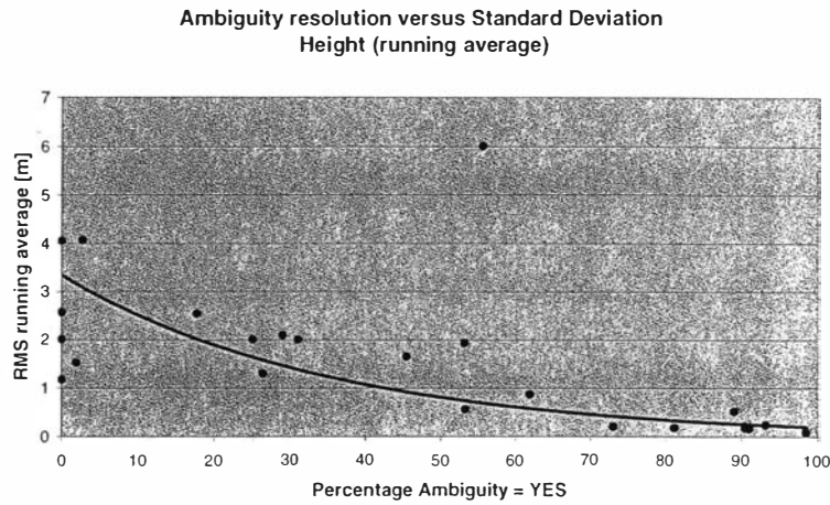
Figure 2: Dependence of standard deviation (height) on ambiguity resolution
