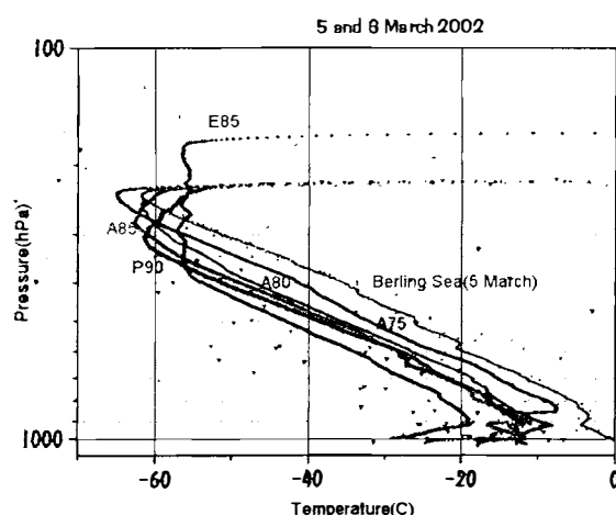
Fig. 2 Temperature profiles from drop sonde measurements along the flight route at Bering Sea, Alaskan side, 75° N, 80° N, 85° N, Pole, 85° N in the European side, on 5 – 6 March 2002.
