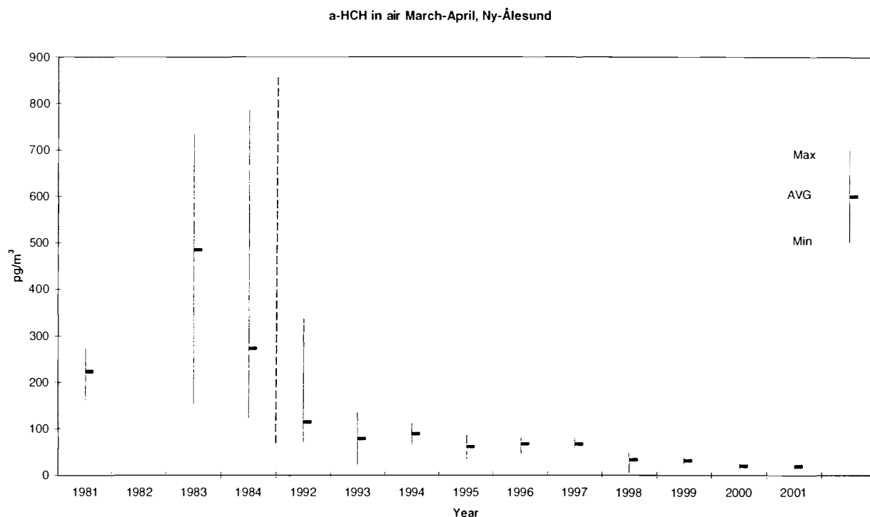
Figure 4: \alpha -HCH in air (March – April) from 1981 – 2001 at Ny-Ålesund
