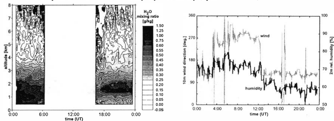
Figure 3: Water vapour mixing ratio observed by KARL (left) and wind and relative humidity from the meteorological station on February 28, 2002.
