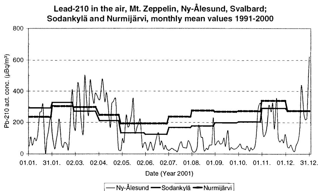
Figure 1. 210 Pb activity concentration (µBq/m 3 ) in the air at Mt. Zeppelin GAW station, Ny-Ålesund, Svalbard in 2001 and monthly mean values at Nurmijärvi and Sodankylä, Finland 1991-2000.
