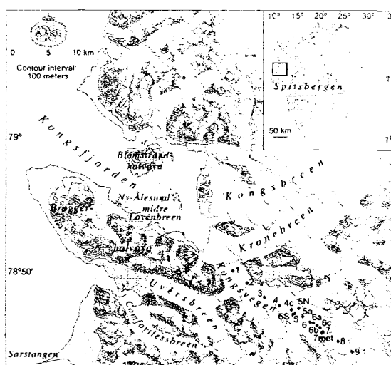
Figure 1: The study area. Core locations are marked on Kongsvegen.
