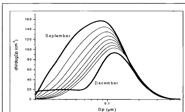
Figure 2 The thick lines show the monthly mean size distributions for September and December. The thin lines represent the calculated change in the aerosol size distribution due to coagulation for each 2 weeks of simulated time. The model was initialized with the September distribution.
