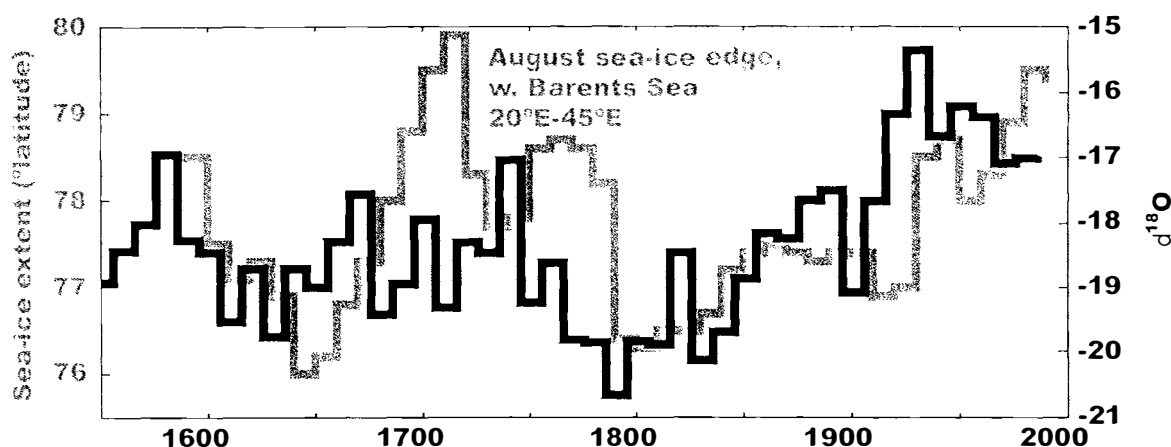
Figure 2. The decadal scale Austfonna \delta^{18}\text{O} record (black) corresponds well to the August sea ice record (grey) from western Barents Sea, compiled with data from whaling ships (Vinje, 2001). This is suggesting that \delta^{18}\text{O} in the precipitation is directly influenced by distance to moisture source in the Austfonna ice core (from Isaksson et al. , submitted).
