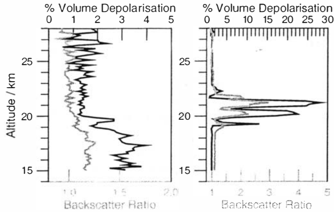
Fig.1: Backscatter Ratio ( grey line ) and volume depolarisation ( black line ) of different solid PSC observations. left: common PSC Ia on January 31, 2000, 10-min-integration at 08:11 UTC. right: PSC Ia with strong depolarisation on January 25, 2000, 10-min-integration at 01:04 UTC.
