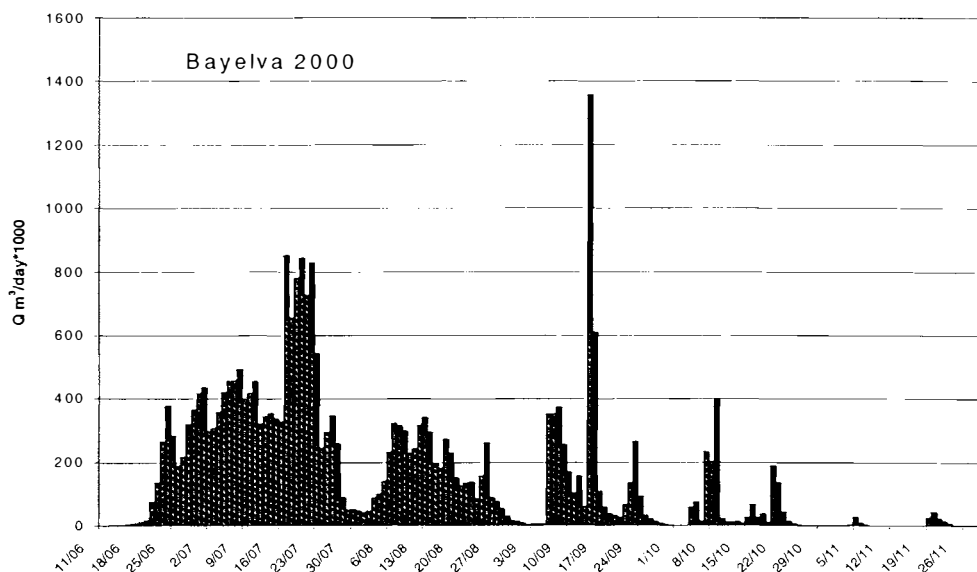
Figure 2. Water volumes discharged in Bayelva in 2000.
