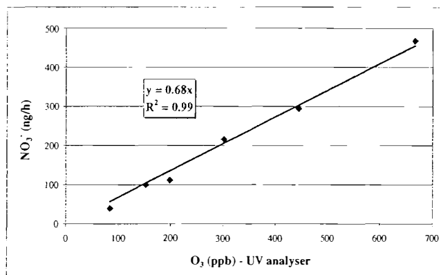
Figure 2 - Relationship between the hourly mean NO 3 - formation onto the diffusive sampler filter and O 3 mixing ratio determined by the UV analyser in laboratory experiments.
