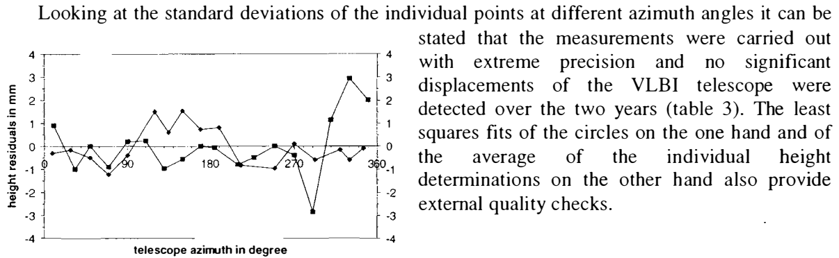
Fig. 4: Residuals of height components
